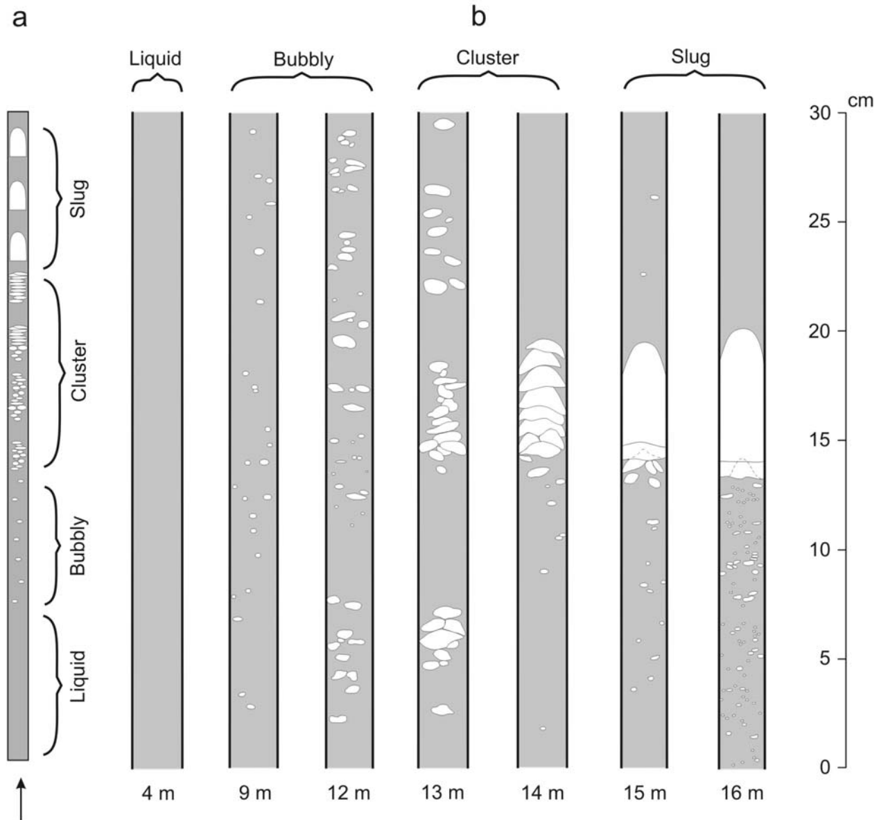
Fig. 2. Fragments of the gas-hydrodynamic regimes originating during ascent of gas-saturated liquid in a vertical transparent hose. (a). Schematic view of location of gas-hydrodynamic regimes in the column; (b). Snapshots of the gas-saturated model liquid flow regimes in the vertical channel. Every shot corresponds to 30 cm window of video recording. All shots of consequently evolving model liquid, were received during one travel of a video camera along the column, with the speed of a moving gas phase.
