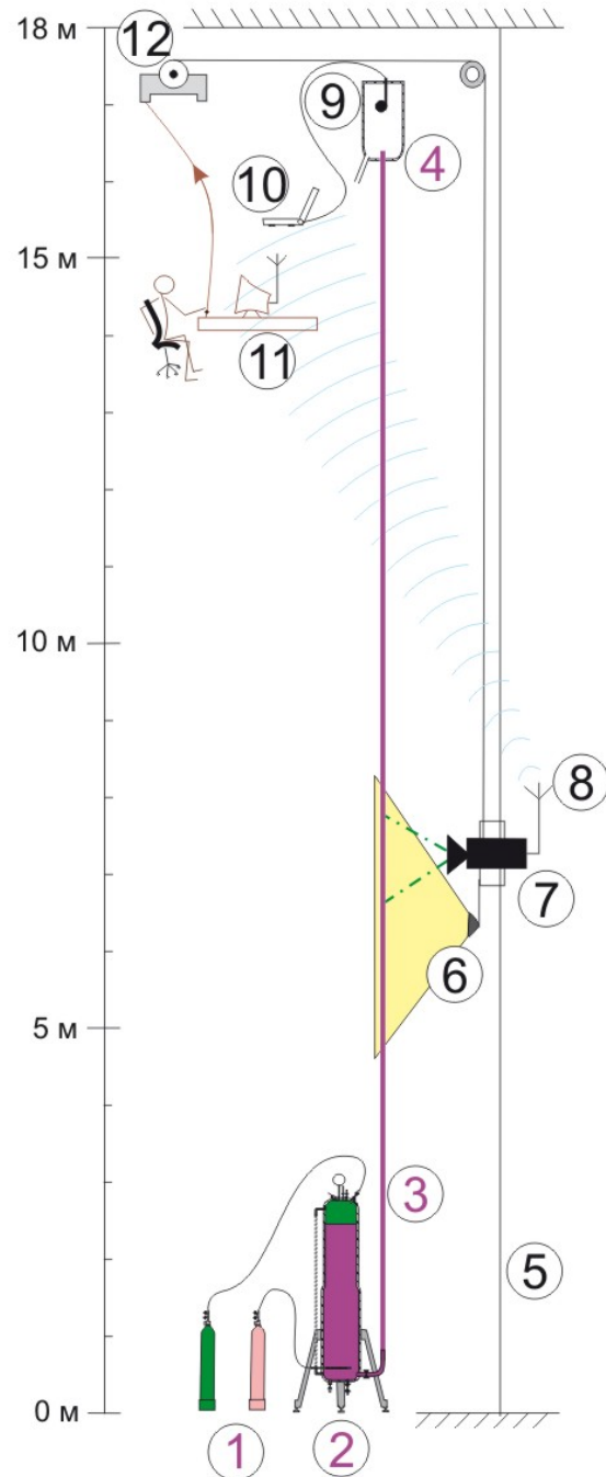
Fig. 1. A complex apparatus for modeling basaltic eruptions – CAMBE.
